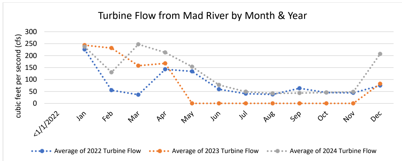
Figure 5: Turbine Flow from Mad River 2022-2024
