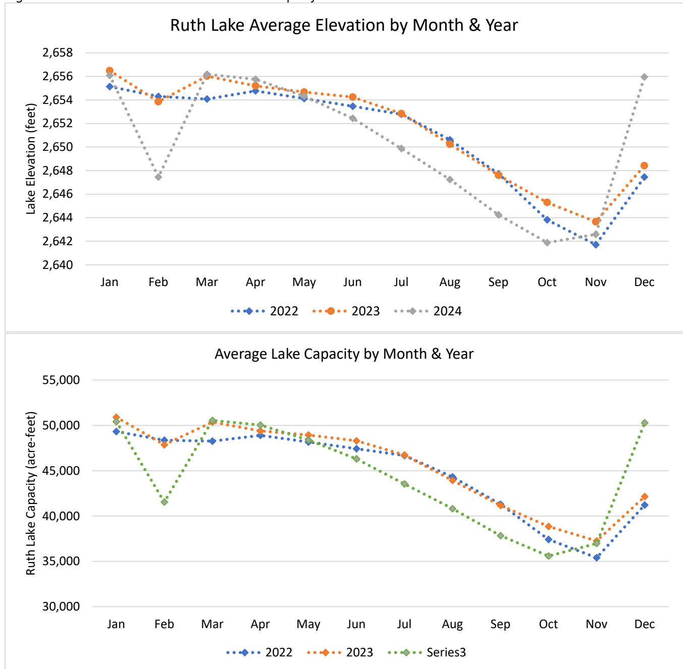
Figure 3: Ruth Lake Reservoir Seasonal Elevation and Capacity 2022-2024
